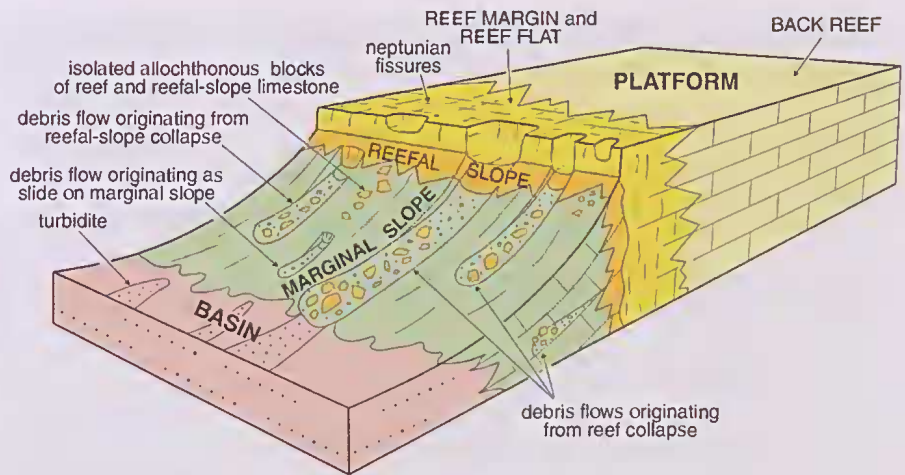
Figure 32 Block diagram illustrating the morphology of the reef complexes and relationships between platform, marginal-slope and basin facies, and associated features.
